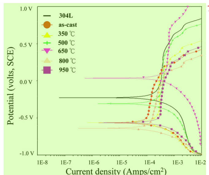
Fig. 5. Potentiodynamic curves of as-cast and aged \text{Al}_{0.5}\text{CoCrFeNi} alloy specimens in 3.5% NaCl solution at 25 °C.
