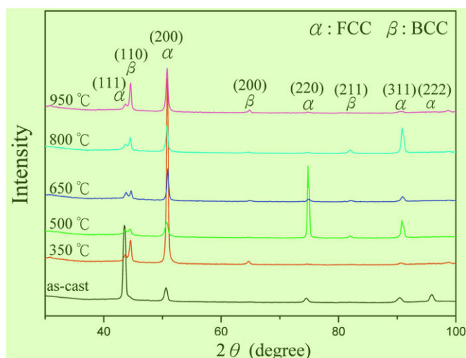
Fig. 2. XRD patterns of Al 0.5 CoCrFeNi alloy processed at various aging temperatures.
